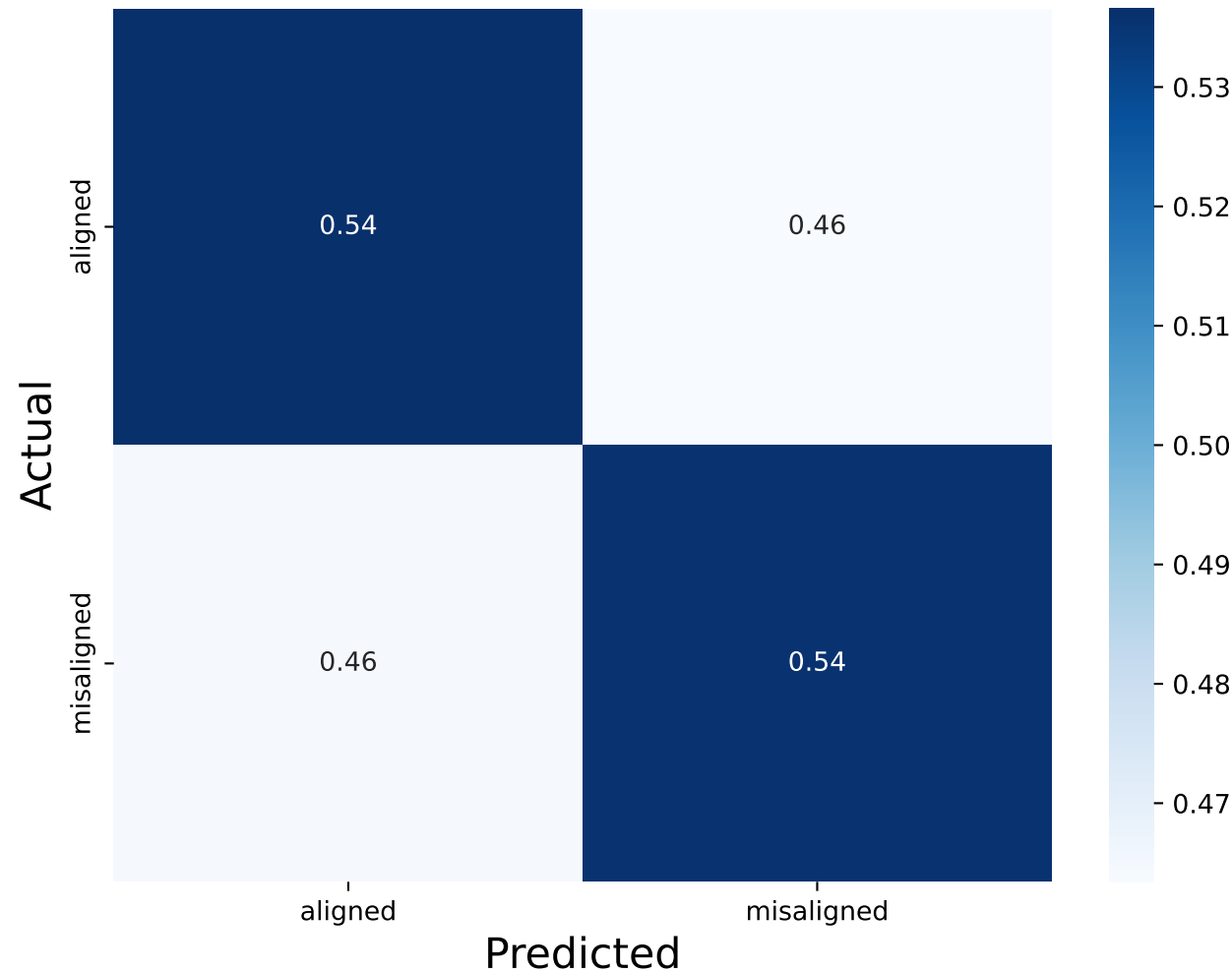
Confusion Matrix of Predicted vs Actual Obliquities (Fraction)
