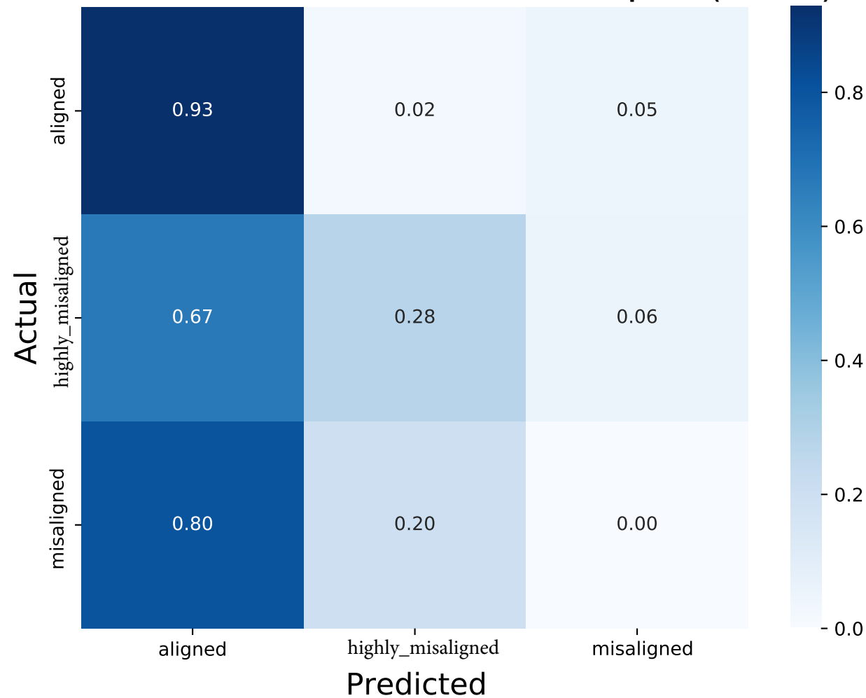
Confusion Matrix of Predicted vs Actual Obliquities (Fraction)
