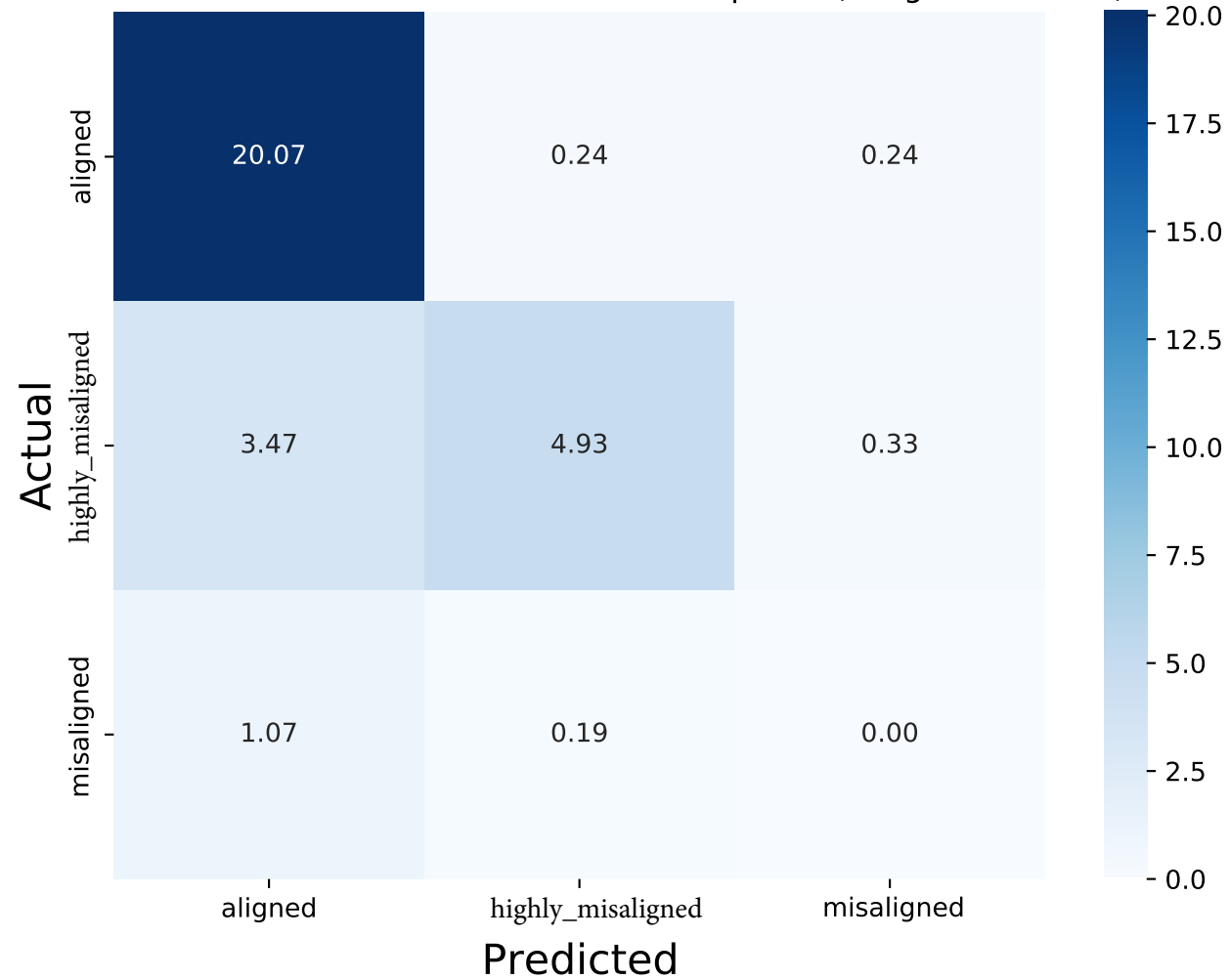
Confusion Matrix of Predicted vs Actual Obliquities (Weighted Counts)
