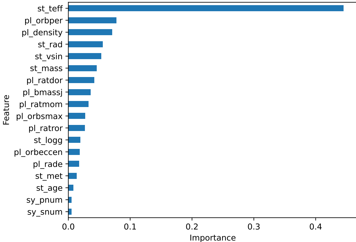
Feature Importances Binary RF Classifier Model
